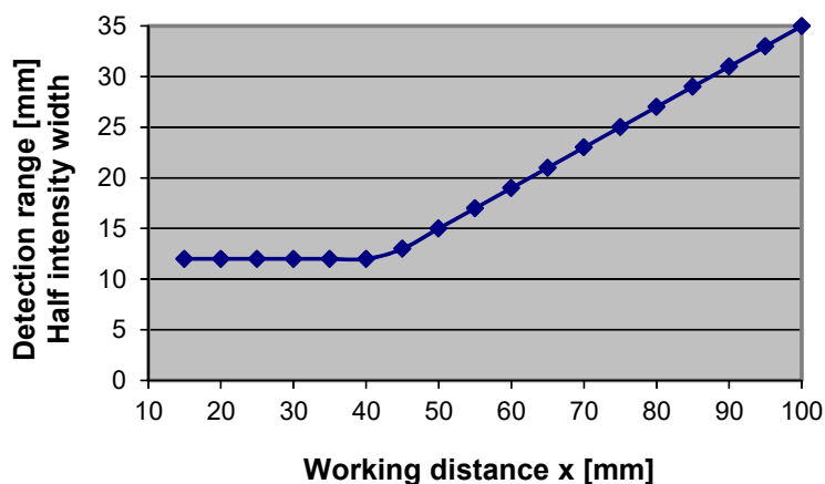
SPECTRO-3-30-FCL-CL Detection range [mm]
